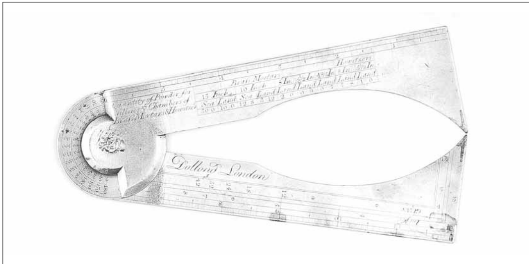
Gunner's calipers by Dollond of London incorporated a one-foot rule divided into inches and tenths of an inch. It was calibrated from 0° to 180° in each direction and was inscribed with calculations of the quantity of powder required for different sizes of brass mortars and howitzers, proof and service charges for brass and iron guns, weight of iron shot etc. In good condition. £775
